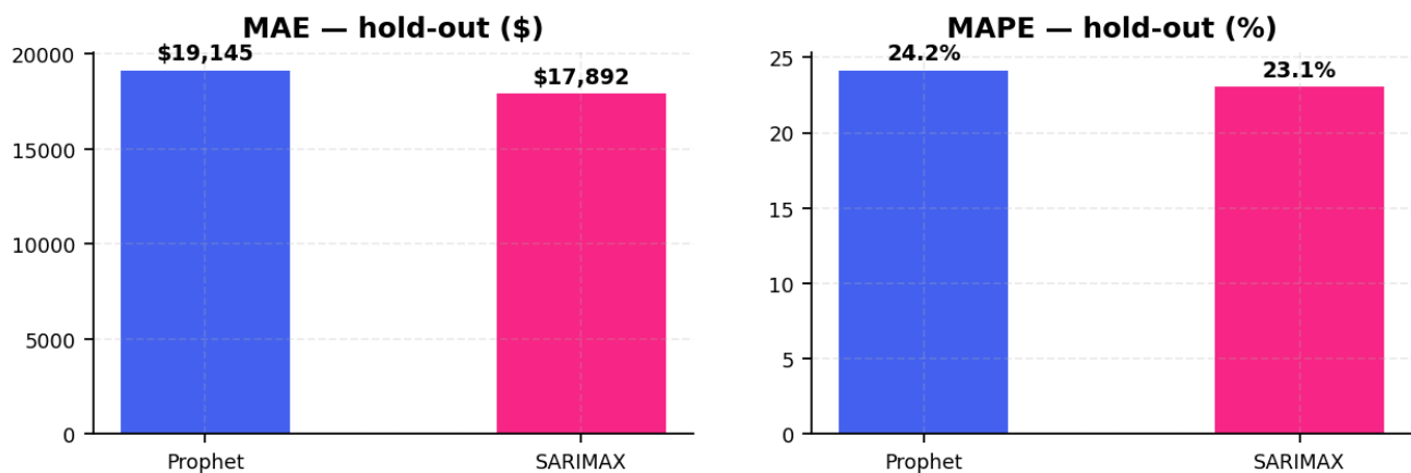
Figure 5 — MAE and MAPE on hold-out evaluation set.
