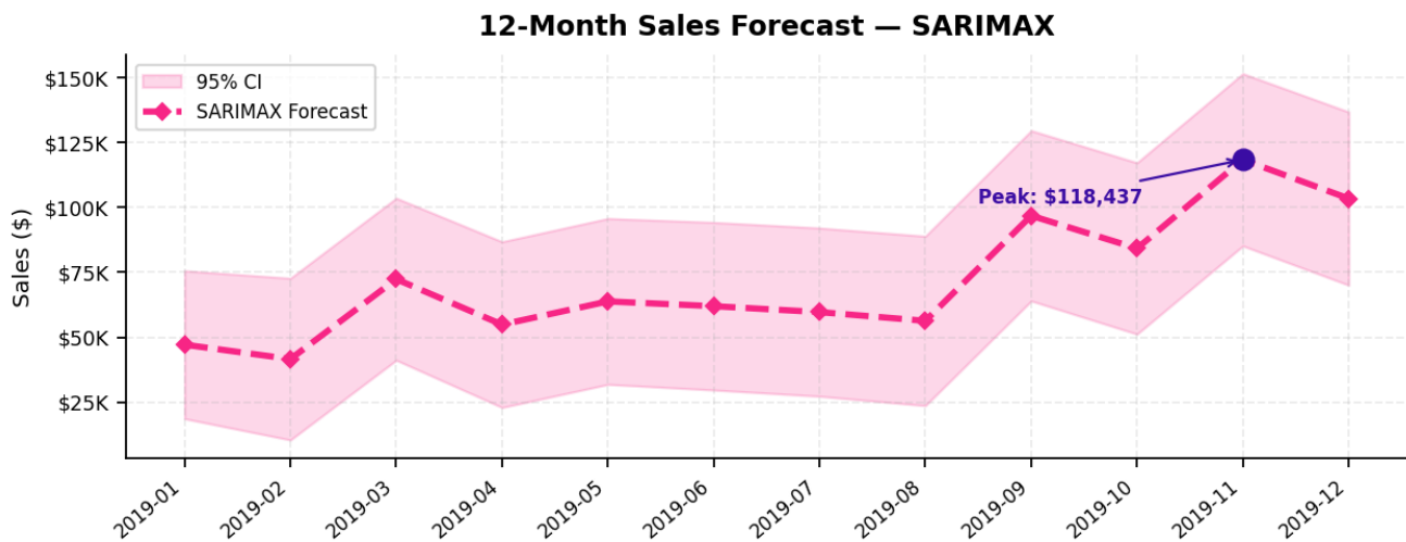
Figure 4 — SARIMAX model forecast for Jan–Dec 2019 with 95% confidence interval.
